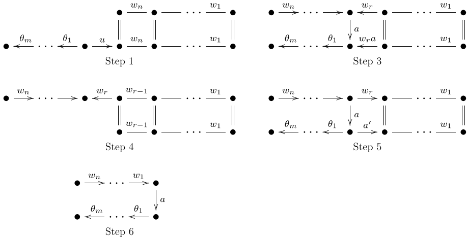
Fig. 1. Diagrams defining the homotopy strings w' and maps f' produced in each step of Algorithm 6.3, with the maximal inverse antipath \theta of Step 8 also added where appropriate.
