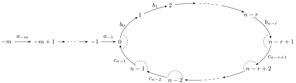
Fig. 2. The bound quiver defining \Lambda(r, n, m) .
