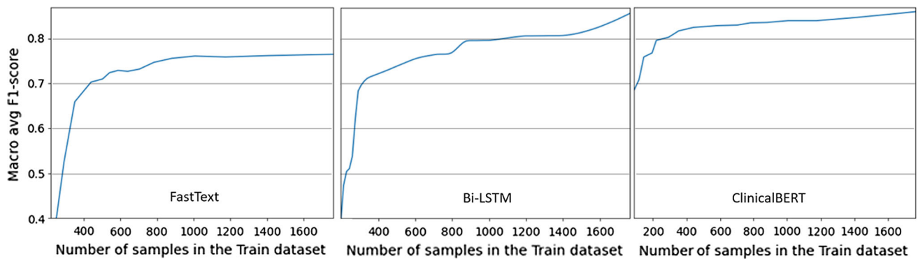
Fig. 1 The trend of Macro-F1 of the FastText, Bi-LSTM and ClinicalBERT classifiers, obtained by varying the number of training samples
