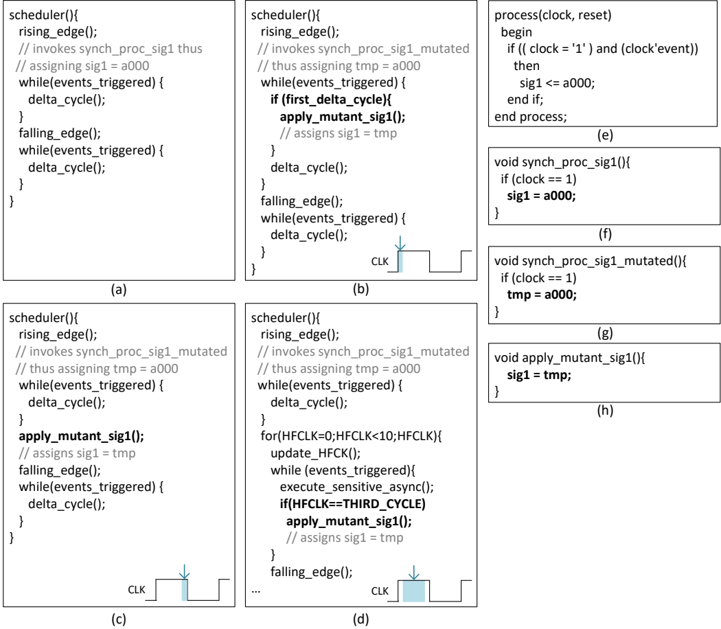
Fig. 9. The proposed mutants for the TLM model: high-level representation of the TLM scheduling without mutants (a), a minimum delay mutant example (b), a maximum delay example (c), and an example of delta delay mutant (d). The snapshots of code apply delays to the assignment \text{sig1} = a000 , for which the figure shows the original VHDL code (e), the corresponding C function (f), and the effect of mutant injection (g-h).
