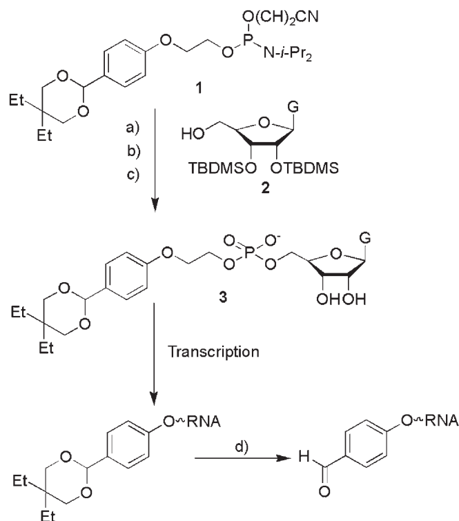
Figure 2. Synthesis of acetal-protected aldehyde-guanosine phosphate 3 . Reagents and conditions: (a) 2 (2.0 equiv), DCI (10 equiv), CH 3 CN, room temperature, 10 min; (b) TBHP (16 equiv), room temperature, 10 min, volatiles removal; (c) TBAF (50 equiv), THF, room temperature, overnight, 16% yield over three steps; (d) 2% TFA in water, room temperature, 15 min, complete deprotection.
