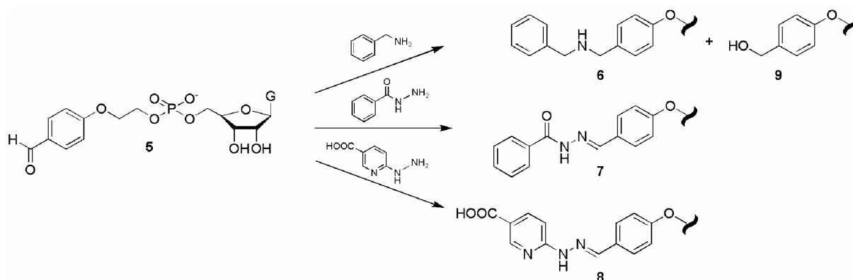
Figure 3. Model reactions performed to establish the conjugation strategy. Benzyl amine, benzoyl hydrazide and 6-hydrazino-nicotinic acid were coupled to unprotected initiator nucleotide 5 . The conjugation with benzyl amine under reductive conditions resulted in the benzyl alcohol derivative 9 as side product.
