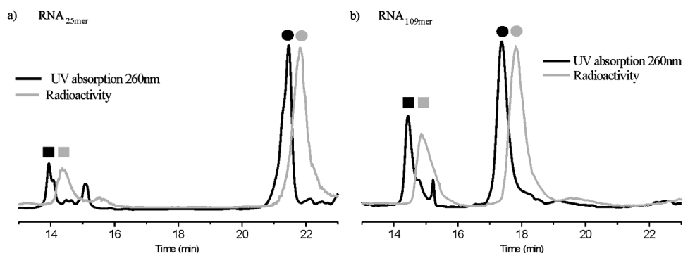
Figure 4. Selective modification of RNA. Incorporation of 3 into a 25mer (a) and 109mer pool (b) RNA by in vitro transcription. Transcription mixtures were analysed by HPLC. UV absorption (black), radioactivity (grey); radioactivity traces are \sim 1 min shifted due to the connection configuration of the radioflow detector. (black squares) Non-initiated transcripts; (black circles) aldehyde-initiated transcripts.
