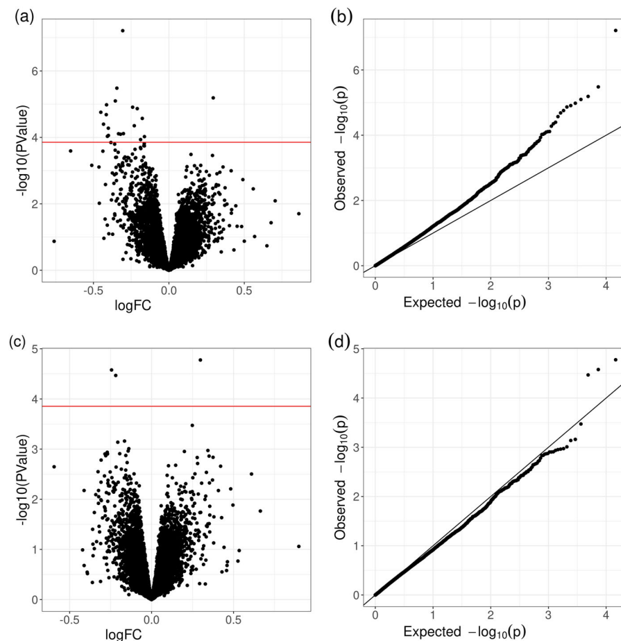
Fig. 1 Differential gene expression analysis. Volcano plots and QQ-plots for the standard model ( a, b ) and for the model with cell composition score as covariate ( c, d ). The inclusion of cell enrichment scores in the DGE model results with a decrease of the inflation rate as measured by the lambda (lambda = 1.23 in ( b ); lambda = 0.975 in ( d )).
