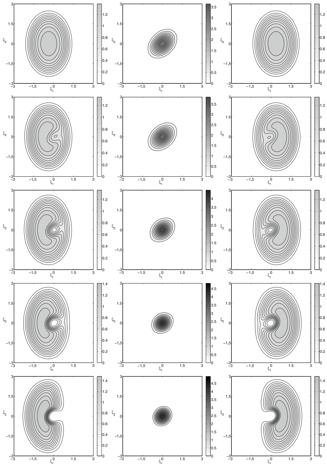
Fig. 4. Contour plots of the ground state ( \varphi^{(1)}(\xi) , \varphi^{(2)}(\xi) , \varphi^{(3)}(\xi) ) of Example 2 (left-right) for \vartheta_{lk} , l \neq k , assuming the values 0, 1.3 \cdot 10^{-6} , 2.5 \cdot 10^{-6} , 5.0 \cdot 10^{-6} and 1.0 \cdot 10^{-5} (top-bottom). The unit length for the function values is 10^3 .
