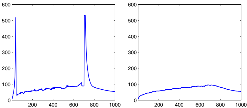
Fig. 2. Number of iterations necessary to compute the ground state of the one-dimensional GPE (2) with the standard harmonic potential U(\xi) = \frac{1}{2}\xi^2 , N = 1 , as a function of \vartheta . The left figure displays the results obtained with the traditional choice \alpha = 10^{-4} , the right figure those obtained with the new strategy (25) for selecting \alpha .
