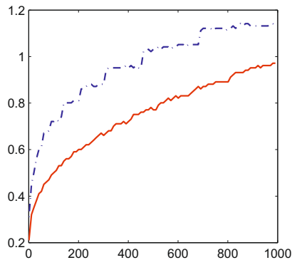
Fig. 1. CPU time in seconds necessary to compute the ground state of the one-dimensional GPE (2) with the standard harmonic potential U(\xi) = \frac{1}{2} \xi^2 , N = 1 , with J = 140 Hermite functions, as a function of \vartheta . The exact Newton method (dashed line) is more expensive than our new strategy (solid line), described in Section 3.
