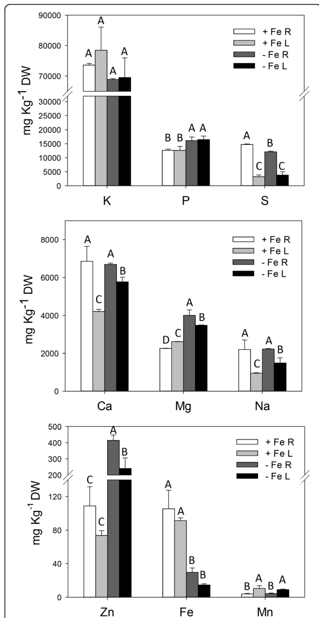
Fig. 2 Macro- and micronutrient concentration [ \text{mg Kg}^{-1} dry weight (DW)] in roots (R) and leaves (L) of 19-day-old maize plants grown under Fe sufficiency (+Fe) or Fe deficiency (-Fe). Data are means \pm SD of three independent experiments (capital letters refer to statistically significant differences among samples for a single nutrient, ANOVA Holm-Sidak, P < 0.05 , n = 3 )
