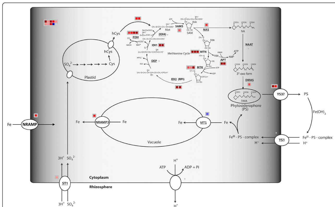
Fig. 4 Transcriptional changes in roots of genes involved in the Methionine cycle/DMA synthesis and Fe acquisition by Fe deficiency. Abbreviations: YS1 = yellow stripe 1; YS3 = yellow stripe 3 ( ZmTOM1 gene, GRMZM2G063306); ST1 = Sulfate transporter 1; SO_4^{2-} = sulfate; Cys = cysteine; hCys = homo-cysteine; FDH = formate dehydrogenase; DEP = methylthioribulose-1-phosphate dehydratase-enolase-phosphatase; IDI1 = 2-keto-methylthiobutyric-acid forming enzyme; IDI4 = putative aminotransferase catalyzing the synthesis of methionine from 2-keto-methylthiobutyric acid; SAMS = S-adenosyl-methionine synthase; MTN = methylthioadenosine/S-adenosyl homocysteine nucleosidase; MTK = methylthioribose kinase; IDI2 = eukaryotic initiation factor 2B-like methylthio ribose-1-phosphate isomerase; NAS = nicotinamine synthase; NAAT = nicotianamine amino-transferase; DMAS = 2'-deoxymugineic acid synthase; APT = Adenosin phosphoribosyltransferase; VIT1 = vacuolar iron transporter 1; NRAMP = natural resistance associated macrophage protein; Regulation = GRMZM2 G057413 (homology to OsIRO2 ), GRMZM2G350312 (homology to OsIRO3 ), GRMZM2G107672 (homology to AtbHLH29 ), GRMZM2G133675 (homology to AtPYE ). Color scale refers to the fold change values of differentially expressed transcripts: red color refers to those transcripts positively regulated by Fe deficiency, while in blue are transcripts negatively regulated Fe deficiency. Adapted from Urbany et al. [39] and Benke et al. [64]
