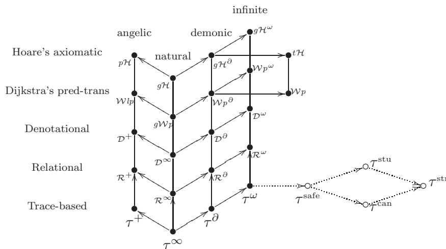
Figure 1. Cousot's hierarchy.
