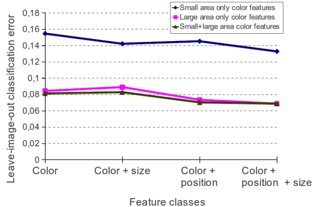
Figure 5. Classification errors obtained with different groups of features.
