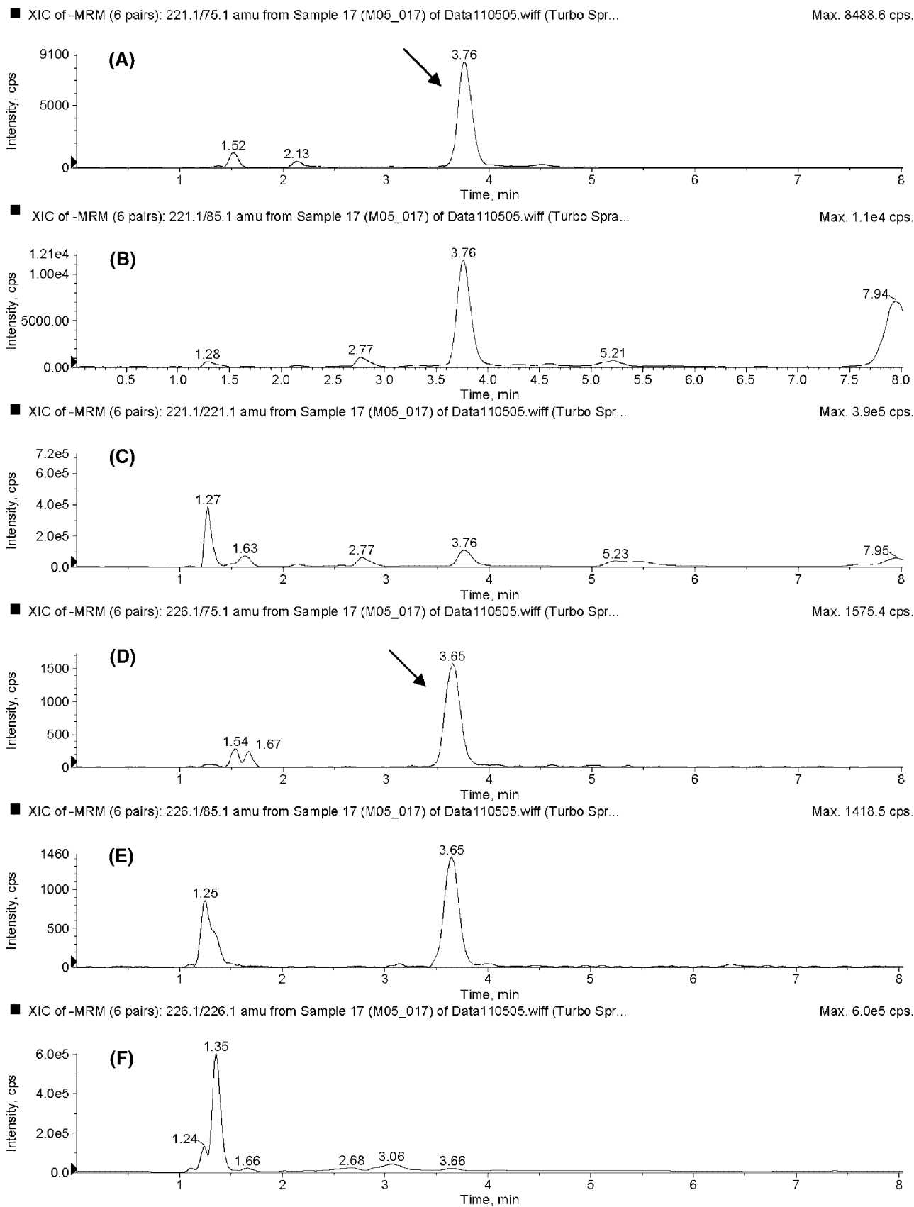
Figure 1. Chromatogram of a real positive hair sample from a withdrawal patient: m/z 221.1 \rightarrow 75.1 (A), 221.1 \rightarrow 85.1 (B), 221.1 \rightarrow 221.1 (C), 226.1 \rightarrow 75.1 (D), 226.1 \rightarrow 85.1 (E), 226.1 \rightarrow 226.1 (F). Concentration of EtG was 434 pg/mg.
