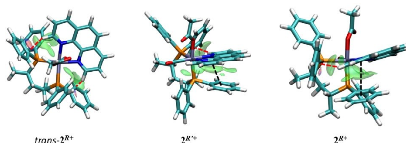
Figure 4. Minimum energy structures with the \delta g^{\text{inter}} isosurfaces (isovalue 0.0055 a.u.) for \text{trans-}2^{R+} and the cis isomers 2^{R'+} and 2^{R+} . Nonbonded interactions: CH–C (red dashed lines), \pi – \pi (black dashed lines).
