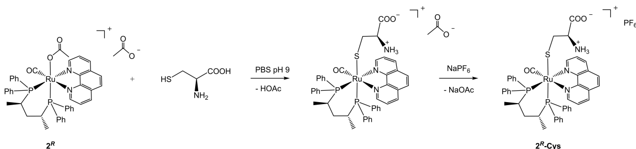
Scheme 4. Reaction of 2^R with (S)-cysteine in water.
