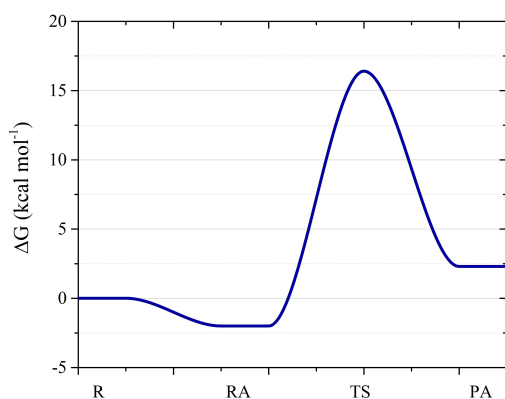
Figure 5. Free energy profile for the hydrolysis reaction leading to the formation of the aquo 2^R\text{-H}_2\text{O}^{++} species. The data for the reaction leading 2^R\text{-OH}^+ are reported in Table S2. The energies of the separated reactants (R) are taken as reference.
