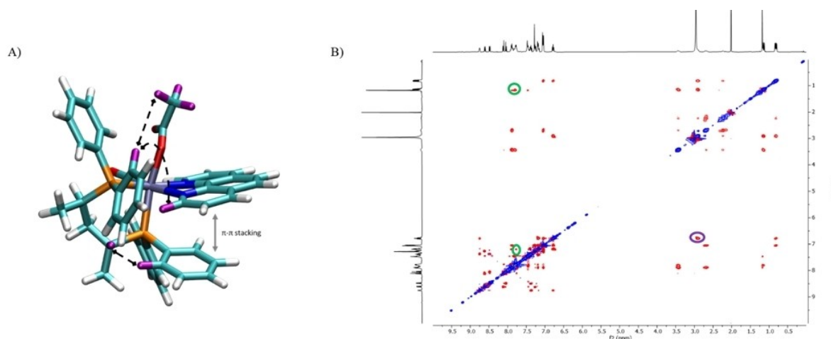
Figure 2. A) Most relevant NOE effects of 2^R displayed by black dashed lines. Involved protons are highlighted in purple; B) NOESY ^1\text{H}\text{-}^1\text{H} NMR spectrum of 2^R in \text{CDCl}_3 . Circled in green: NOE effects of the phenyl protons at \delta 7.78 ppm with both the acetate methyl group at \delta 1.19 ppm and the phenanthroline ortho proton at \delta 7.18; Circled in purple: NOE effects between the chiral CH proton at \delta 2.91 ppm and the two phenyl ortho protons at \delta 6.79 ppm.
