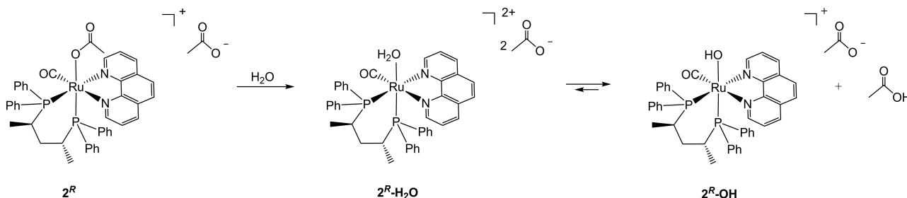
Scheme 3. Formation of the aquo and hydroxo complexes from 2^R in water.
