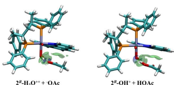
Figure 6. Minimum energy structures for the PA of aquo 2^R\text{-H}_2\text{O}^{++} + \text{OAc}^- and the hydroxo 2^R\text{-OH}^+ + \text{HOAc} complexes. \delta g^{\text{inter}} isosurfaces (isovalue 0.0055 a.u.) in green.
