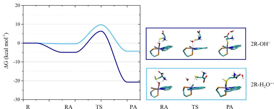
Figure 8. Left: reaction energy profiles in acidic-neutral conditions for the reactions between (S)-cysteine and 2^R\text{-H}_2\text{O}^{++} (light blue), 2^R\text{-OH}^+ (blue). Right: structures of the RA, TS and PA (some atoms were removed for clarity, complete structures in Figure S35).
