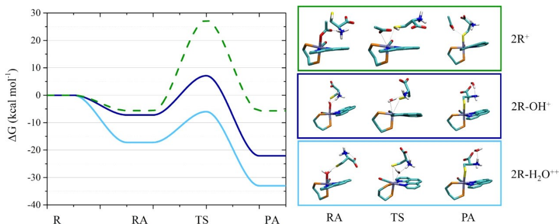
Figure 7. Left: free energy profiles in basic condition for the reactions of the thiol-deprotonated (S)-cysteine with 2^R\text{-H}_2\text{O}^{++} (light blue); 2^R\text{-OH}^+ (blue). The energy profile for the reaction between zwitterionic (S)-cysteine and 2^R is also reported (green dashed line). Right: structures of the RA, TS and PA (some atoms were removed for clarity, complete structures in Figure S34).
