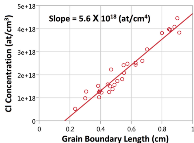
Fig. 17. Total chlorine concentration (atoms/cm 3 ) measured by ToF-SIMS shows a linear relationship with the grain boundary length (cm) measured by EBSD within a fixed 2D fixed field of view. Image from Ref. [199] copyright IEEE and reused by the original author with permission.
