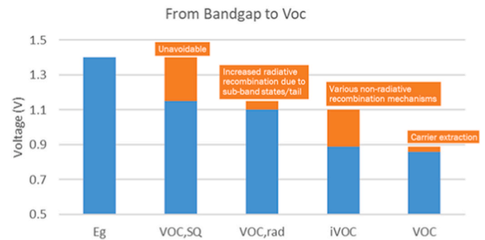
Fig. 12. Estimated breakdown of V_{OC} losses in state of the art As-doped, Se-alloyed cells. Proceeding from left to right, the SQ-mandated losses, sub-gap radiative losses, non-radiative losses, and energy-level-alignment losses are successively subtracted to move from the cell effective bandgap near 1.4 eV to measured V_{OC} below 900 mV.
