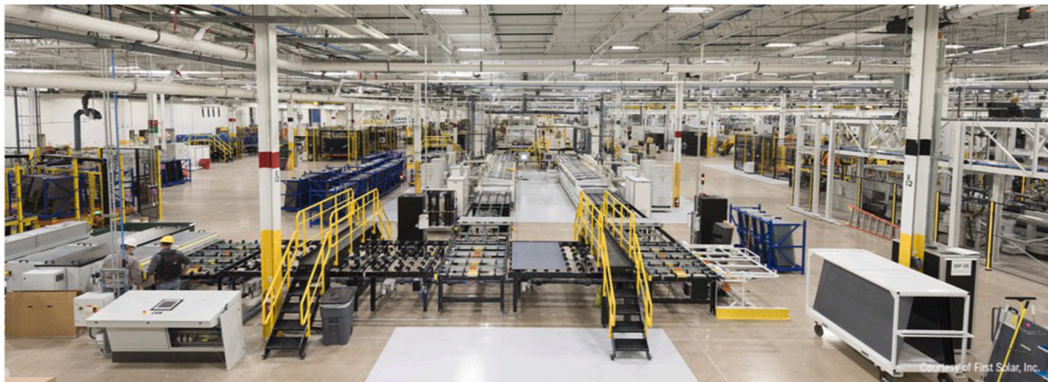
Fig. 7. View of a First Solar manufacturing line. A grey rectangular Series 6 module is visible in the foreground on the conveyance system between the two walkover paths with yellow railings and two workers are present to the left for scale. Hundreds of other nearly-finished modules are visible in the blue metal racks to either side. It is remarkable to note that high-efficiency CdTe modules are produced in factories in which they are transported in open air between process steps rather than e.g. in a cleanroom. Image courtesy of First Solar.
