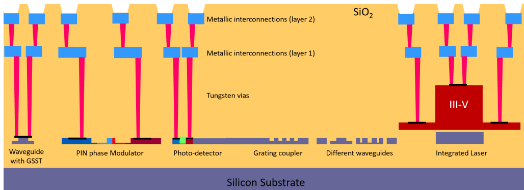
Fig. 2. Cross-section of the augmented silicon photonics platform in NEUROFULS. PCMs such as GSST (left side) and III-V materials (right side) are integrated on top of waveguides. Two layers of interconnects will be available for routing purposes.
