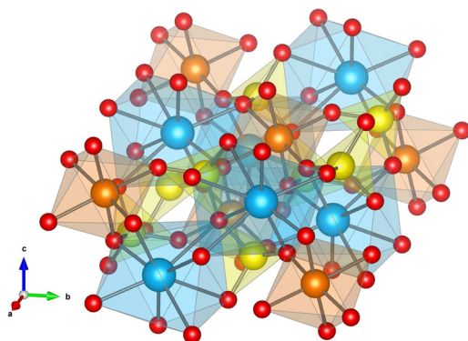
Fig. 1 Diopside, unit cell: \text{Mg}^{2+} orange, \text{Ca}^{2+} cyan, Si yellow and O red. M1 sites are composed each of six \text{Si}=\text{O} groups that form a square bipyramidal shape (orange octahedron) accommodating the \text{Mg}^{2+} cations. The \text{Ca}^{2+} cations, interacting with oxygen of \text{Si}-\text{O} at the bridge site ( \text{Si}-\text{O}_{\text{br}} ) and the nearest \text{Si}=\text{O} , fill the larger M2 sites (cyan). The \text{SiO}_4 tetrahedral groups are in yellow.
