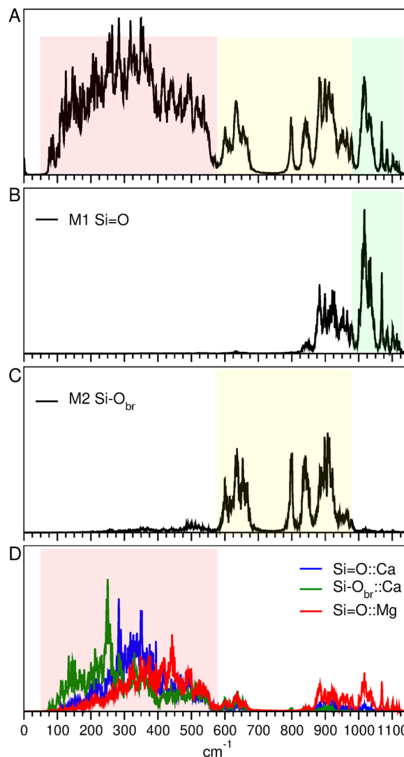
Fig. 2 Calculated VDOS for pure diopside. (A) VDOS evaluated taking into account all atoms. The colored area highlights the regions of the vibrational spectra of diopside: green 1000\text{--}1200\text{ cm}^{-1} , yellow 600\text{--}1000\text{ cm}^{-1} and red 100\text{--}600\text{ cm}^{-1} . (B) pVDOS for Si=O stretching involved in two M1 and two M2 selected sites. (C) pVDOS for Si-O br stretching in the selected sites. (D) pVDOS for stretching between oxygen and the metal cation of M1 (Si=O::Mg 2+ , red line) and M2 (Si=O::Ca 2+ , blue line; Si-O br ::Ca 2+ , green line).
