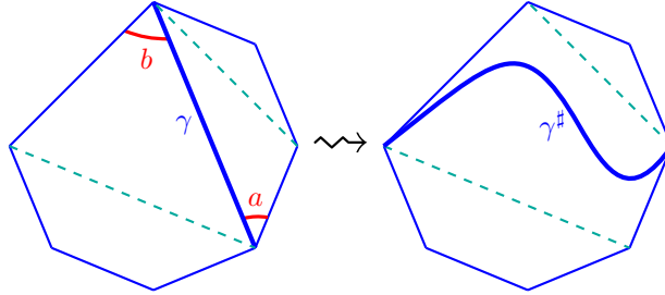
FIGURE 6. Refinement of a flip \mathbb{A} \xrightarrow{\gamma} \mathbb{A}_\gamma^\sharp (collision case)
