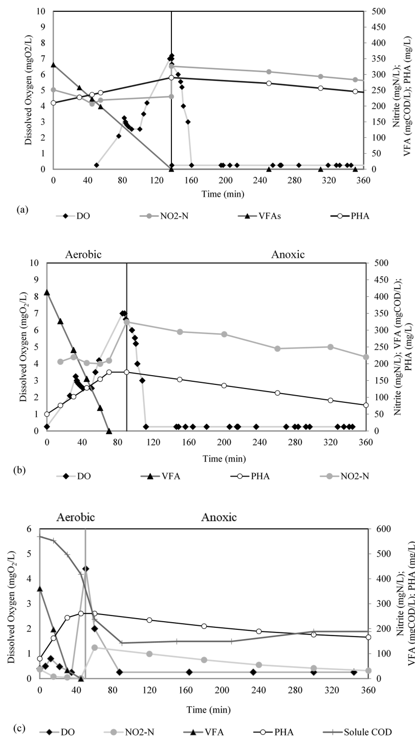
Figure 5. Typical profiles of electron acceptors (dissolved oxygen and nitrite), VFAs, and PHAs during the feast and famine phases of (a) period 1, (b) period 2, and (c) period 3.
