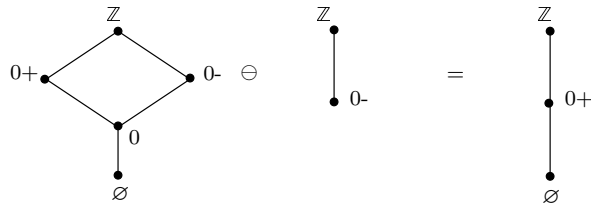
Fig. 2.8. Abstract domain complementation
