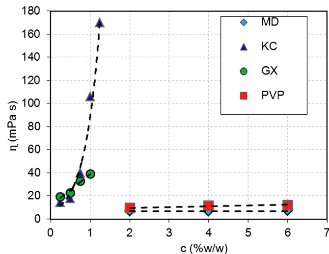
Fig. 1. Dispersion viscosity for the selected binders as a function of the concentration in water.
