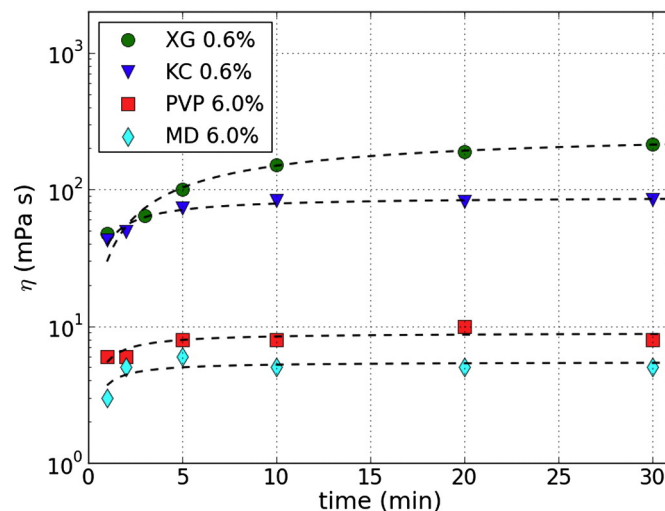
Fig. 2. The thickening tendency of the selected polymers is the result of a combination of different rate processes with different kinetics (dispersion, hydration, gelification). In general, polymers giving lower viscosity dispersions (PVP, MD) hydrate faster than those yielding greater viscosity (KC, XG).
