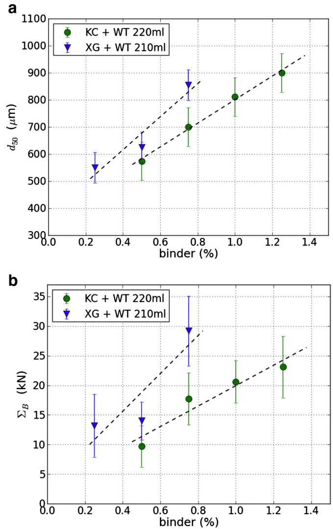
Fig. 4. Dependence of a) median diameter d_{50} and b) granule strength \Sigma_B on binder amount for KC and XG binder based granules.
