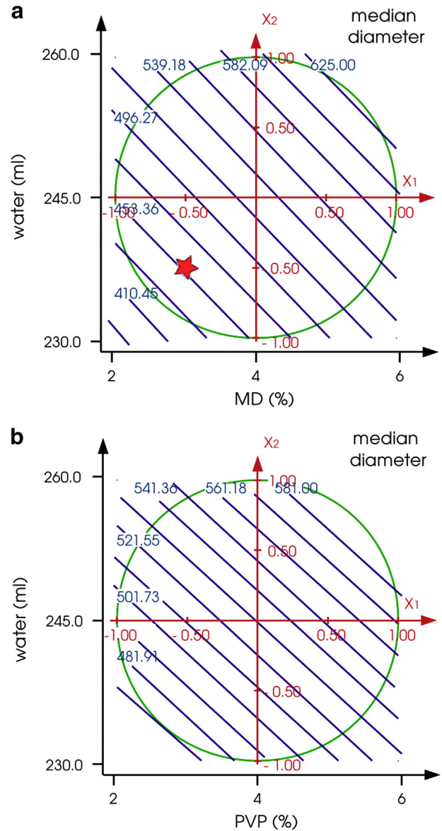
Fig. 3. Two dimensional representation of the isoresponse planes obtained from the multivariate regression analysis for the selected variable d_{50} : a) MD based granules. The star represents the additional granulation performed to validate the model; b) PVP based granules.
