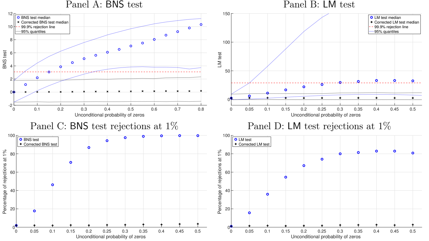
FIGURE 2: Quantiles (median, 5% and 95%) of daily jump tests in their original and corrected version, with the 99.9% rejection line, on simulated 5-minute returns, as a function of the generated probability of staleness. Panel A: BNS test. Panel B: LM test. Panel C and D report rejection rates of BNS test and LM test respectively at confidence level 1%.
