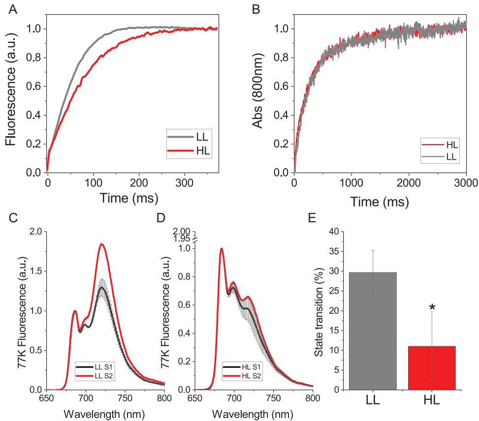
Fig. 1. Functional antenna sizes of PSI and PSII, and the state transitions. (A) Chl a fluorescence emission kinetics of whole cells grown in low light (LL) or high light (HL) treated with DCMU (representative of three independent biological replicates), related to the light-harvesting efficiency of PSII. (B) Kinetics of PSI reaction center oxidation followed by pump-probe differential absorption at 800 nm measured in whole cells treated with DCMU, methyl-viologen, and ascorbate (representative of three independent biological replicates) as described in the Materials and methods. (C and D) Chl a fluorescence emission spectra measured at 77K for cells grown in LL (C) or HL (D) in state 1 (S1) or state 2 (S2); S1 was induced in LL ( \sim 5 \mu\text{mol m}^{-2} \text{s}^{-1} ) with 10 \mu\text{M} DCMU to oxidize the plastoquinone pool, while S2 was induced by adding 250 \mu\text{M} sodium azide to inhibit mitochondrial respiration and reduce the plastoquinone pool. (E) Extent of state transition retrieved from fluorescence emission spectra reported in (C) and (D) from the maximum fluorescence emission at 720 nm as (\text{FS2}-\text{FS1})/\text{FS2} . Error bars are reported as SDs ( n=3 ). * P<0.05 for HL versus LL.
