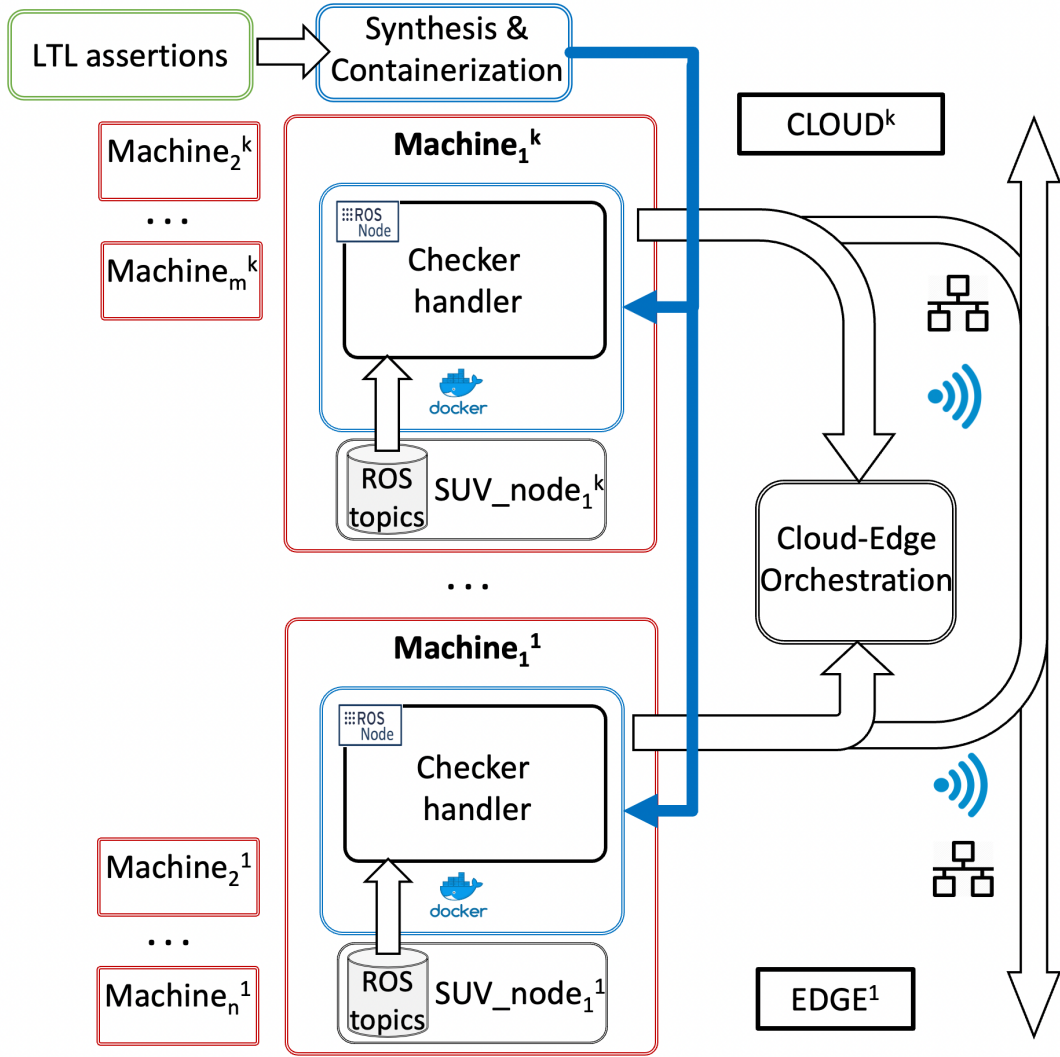
FIGURE 7.1: Verification architecture.
