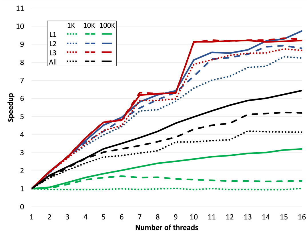
FIGURE 5.14: Speedup of the 3-level parallelisation
