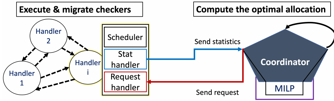
FIGURE 7.4: Orchestrator's architecture.
