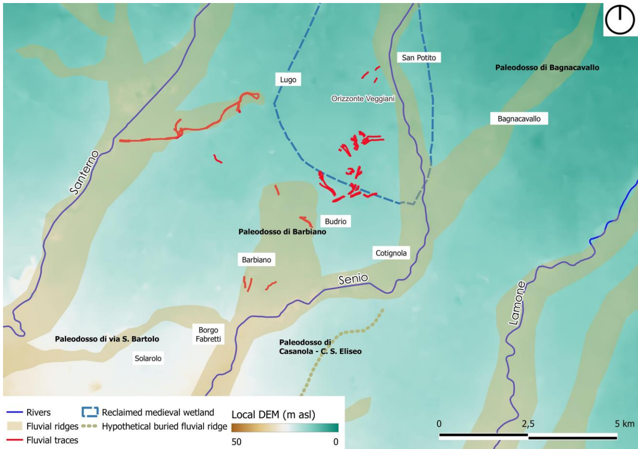
Fig. 2. Geomorphological map of the territory of Cotignola with rivers, fluvial ridges (Italian names in bold) 21 , hamlets and towns mentioned, the extension of the Orizzonte Veggiani and main fluvial traces mapped by remote sensing. Visualisation of a 10m resolution local DEM as basemap 22 (author M. Abballe).
