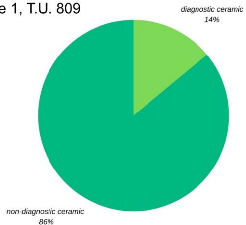
Fig. 8. Above, site 1, T.U. 871 (Cunio), quantification of the archaeological finds collected, histogram; below, pie charts representing the percentages of diagnostic and non-diagnostic ceramic in T.U. 871 and T.U. 809 in Budrio (author A. Ferrari).
