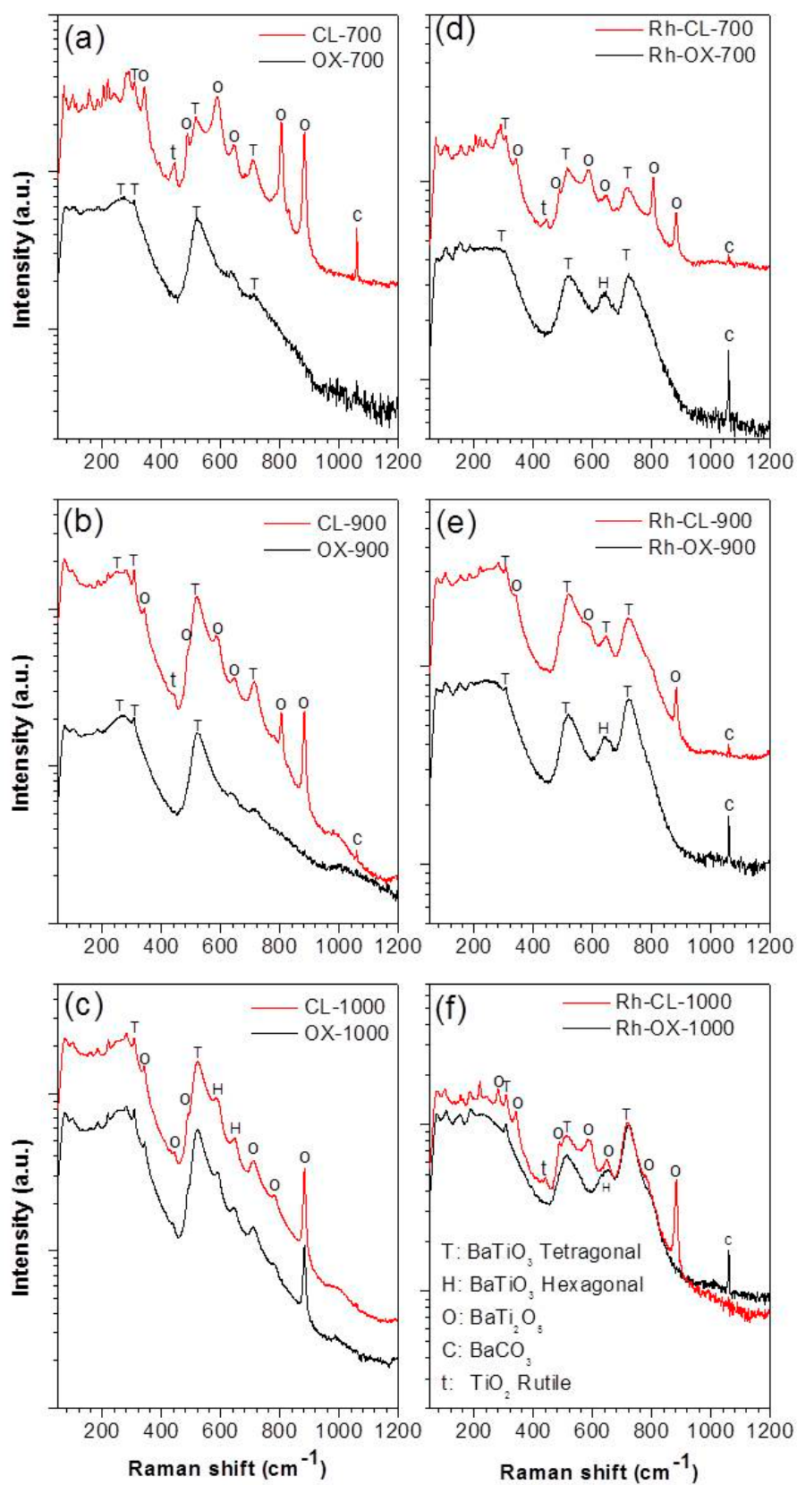
Figure 5. Raman spectra of undoped \text{BaTiO}_3 (a–c) and Rh doped \text{BaTiO}_3 (d–f) prepared by oxalic and classic routes.
