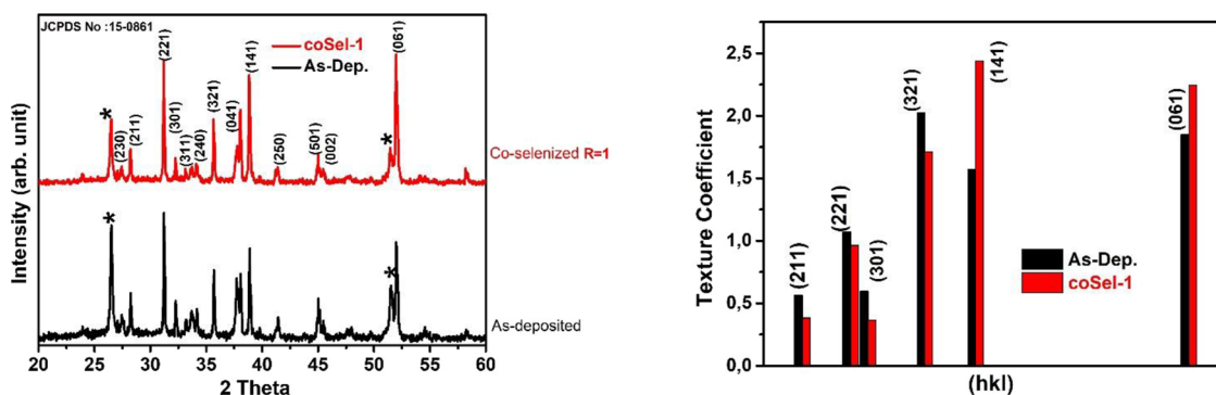
Figure 1. XRD spectra and TC of the as-deposited and co-selenized samples.
