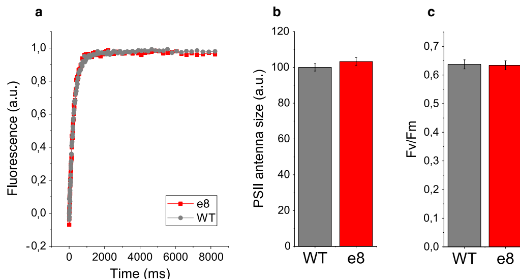
Fig. 2 PSII functional antenna size and PSII maximum quantum yield. a Fluorescence induction kinetics of PSII antenna size of wild type and selected mutant. b PSII functional antenna size expressed as the reciprocal of the time required to reach 2/3 of the maximum fluorescence emission, \tau_{2/3}^{-1} (%). c PSII maximum quantum yield calculated as (F_M - F_0)/F_M from basal chlorophyll fluorescence in the dark ( F_0 ) and maximum chlorophyll fluorescence induced by a saturating pulse ( F_M ). The statistical analysis of the results obtained was performed by unpaired two-sample t-test ( n = 4 , no statistically significant difference being p -value = 0.09 for PSII functional antenna size and p = 0.78 for F_v/F_m values)
