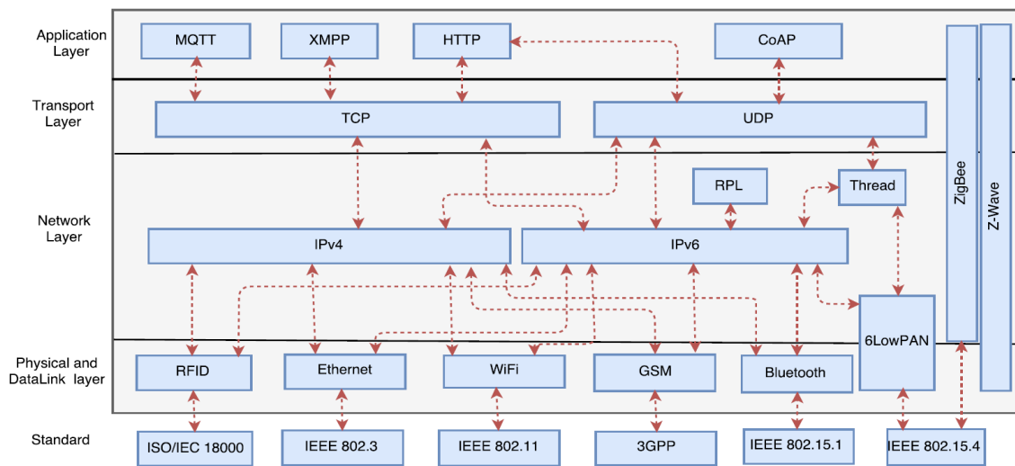
Figure 4: IoT Network Stack and Standards
